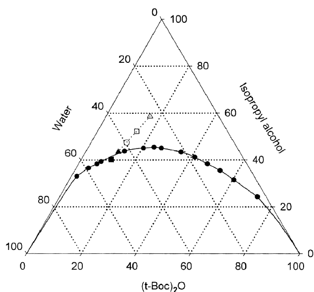
Fig. 4. Phase diagram for the ternary system of \text{Boc}_2\text{O} , Isopropyl alcohol (IPA) and Water. ●: measured solubility, △: 9 equivalency of KOH, □: 10 equivalency of KOH, ○: 11 equivalency of KOH, ▲: 12 equivalency of KOH, ■: 13 equivalency of KOH.
